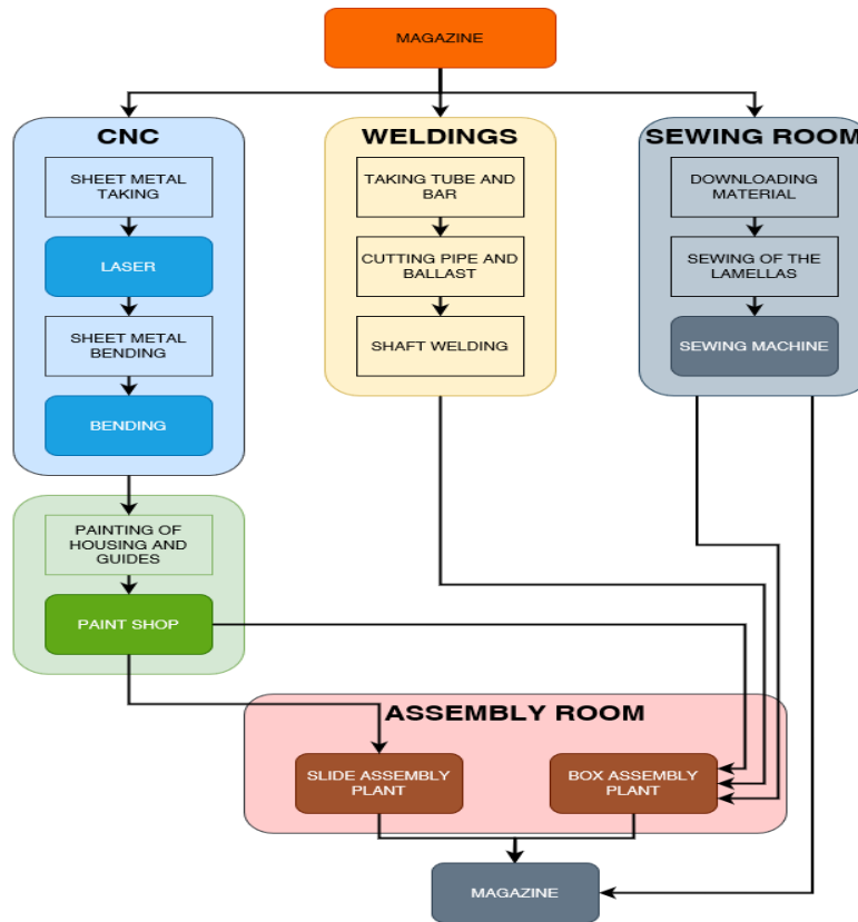
Figure 3 Manufacturing process scheme (A3)
