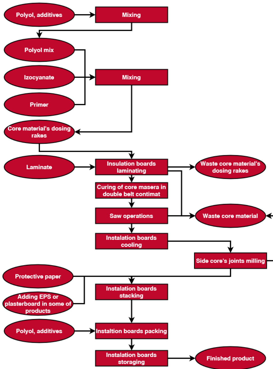
Figure 2. The scheme of Thermano insulations production process by Balex Metal Sp. z o.o.
