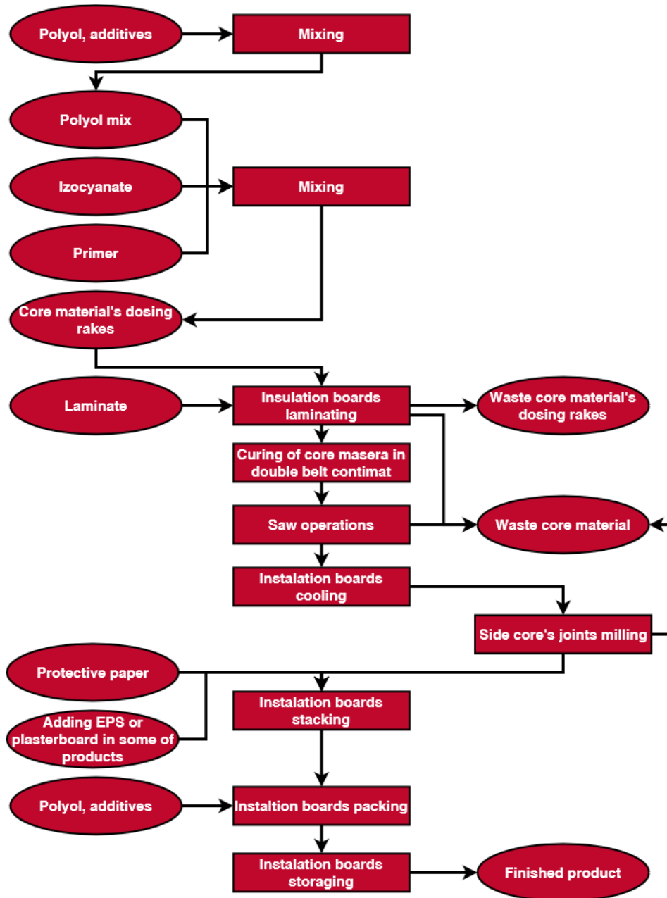
Figure 2. The scheme of Thermano Floor production process by Balex Metal Sp. z o.o.
