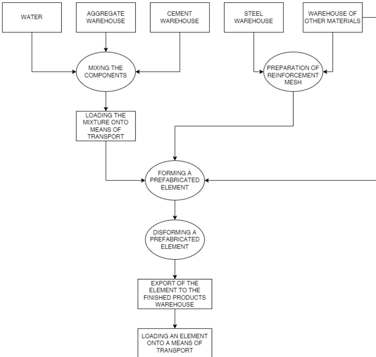
Figure 2. Diagram of the manufacturing process of prefabricated single- and multi-layer wall elements
