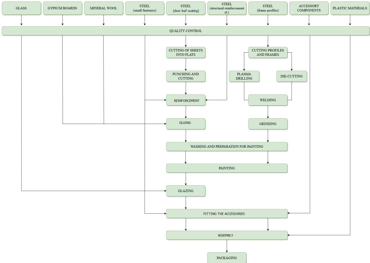
Fig. 1. A basic scheme of steel doors manufacturing process
