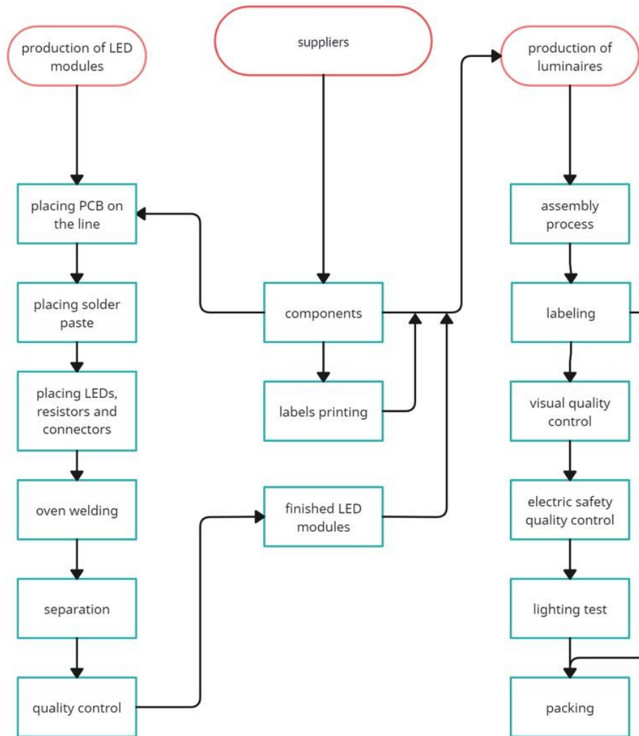
Fig. 3. A basic scheme of LED luminaire/aluminium product manufacturing process
