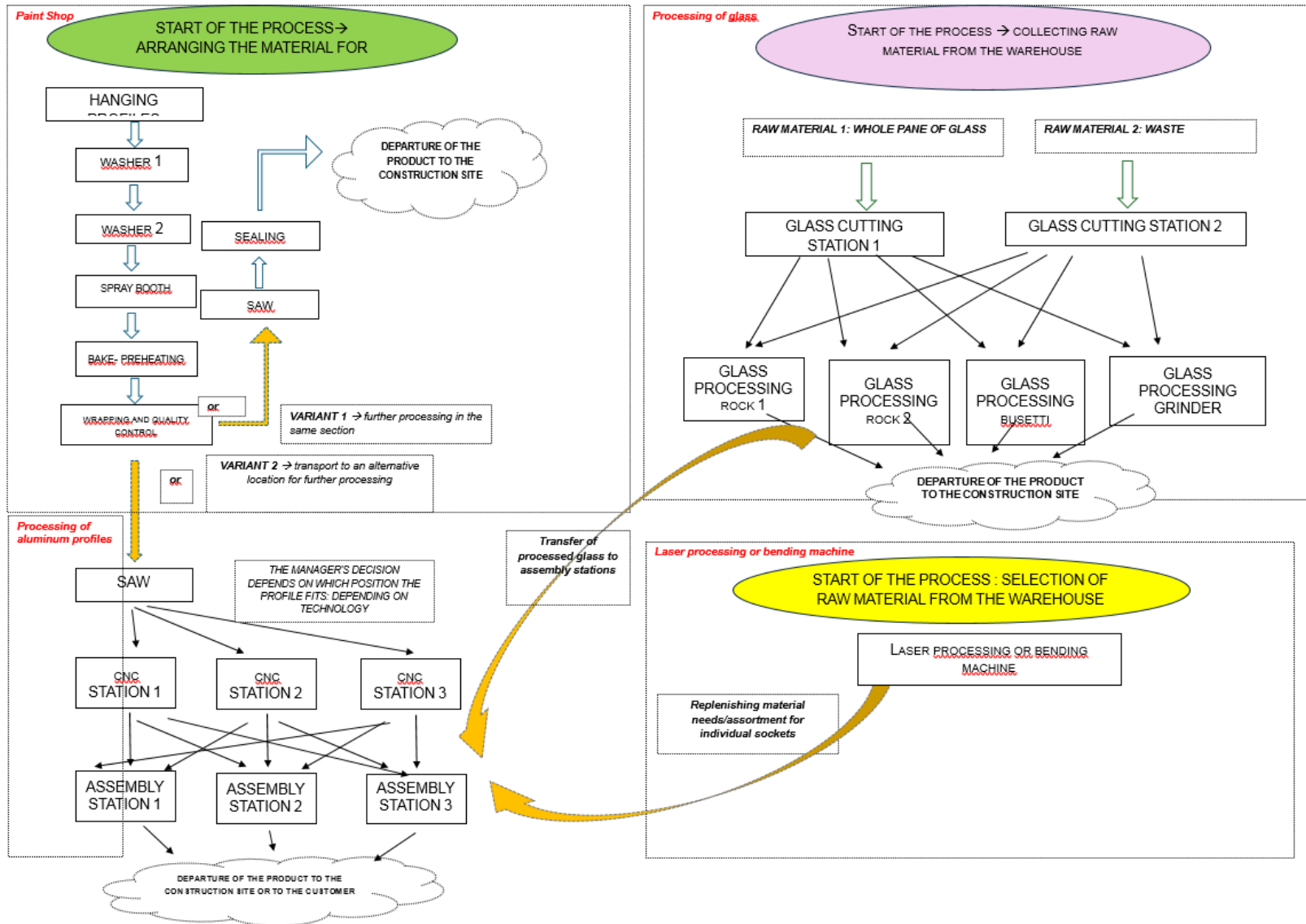
Fig. 3. A scheme of aluminium-glass Vitrintec systems production by VITRINTEC Sp. z o. o.
