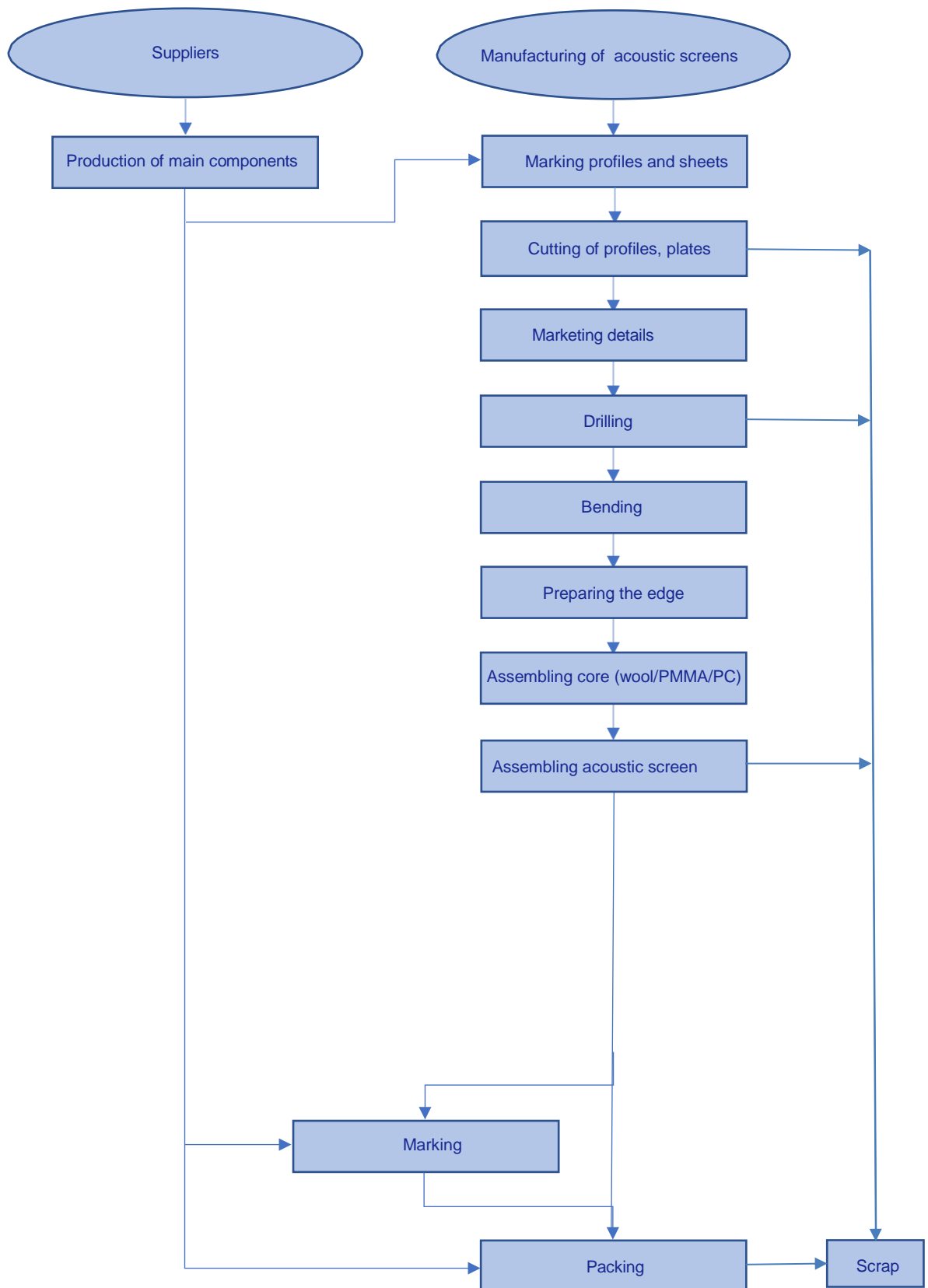
Figure 1. A basic scheme of CALVERO® acoustic screen product manufacturing process.
