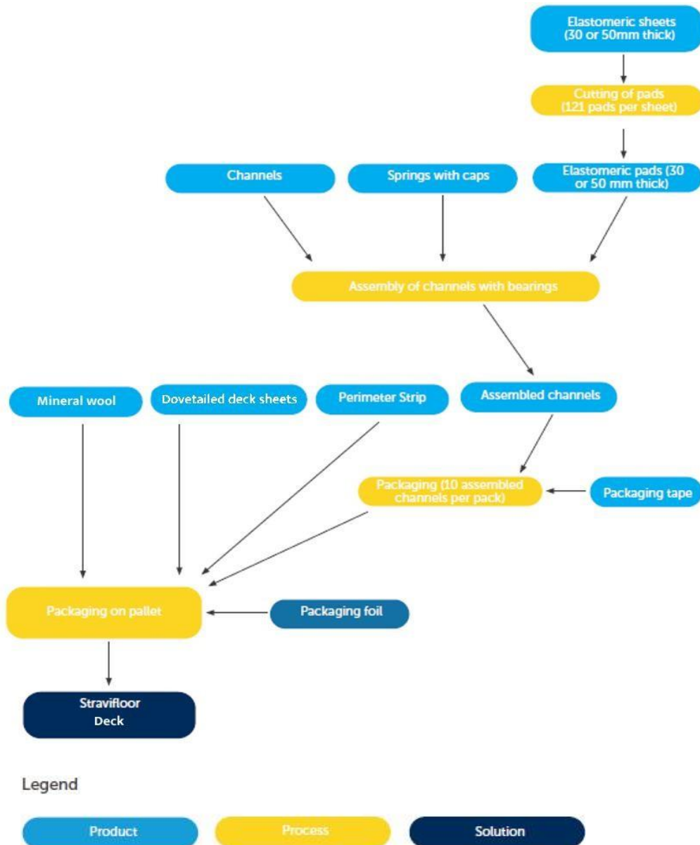
Figure 2. Diagram of the manufacturing process of the Stravifloor Deck solution in CDM Stravitec Warehouse in Wavre, Belgium
